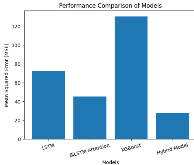
Fig. 4. Performance Comparison of Models
