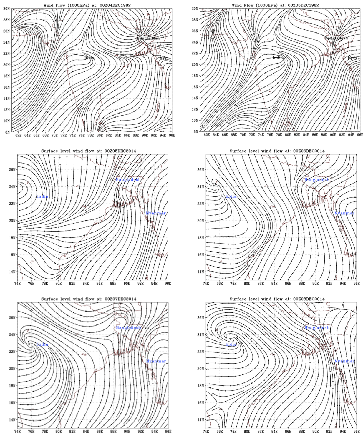
Fig.9: Wind flows at 1000hPa level in 1982 and 2014
