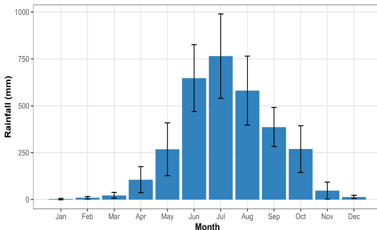
Fig. 3: Monthly distribution of rainfall in Bandarban district during 1981-2025
