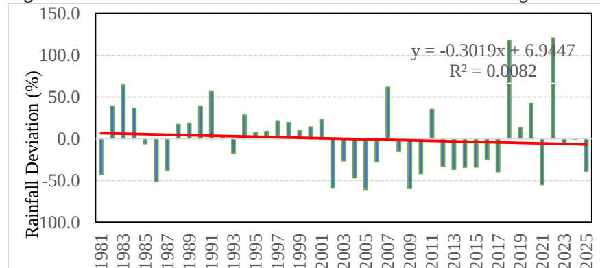
Fig. 9: Deviation of Pre-monsoon Rainfall in Bandarban district during 1981-2025
