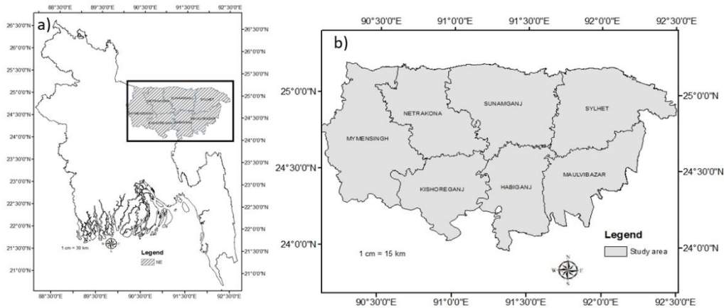
Figure 1: Study area a) Bangladesh b) Northeast region.
