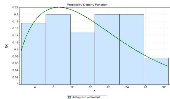
Fig.7(b): PDF of Weibull Distribution of \text{MinT} \leq 10^\circ\text{C}
