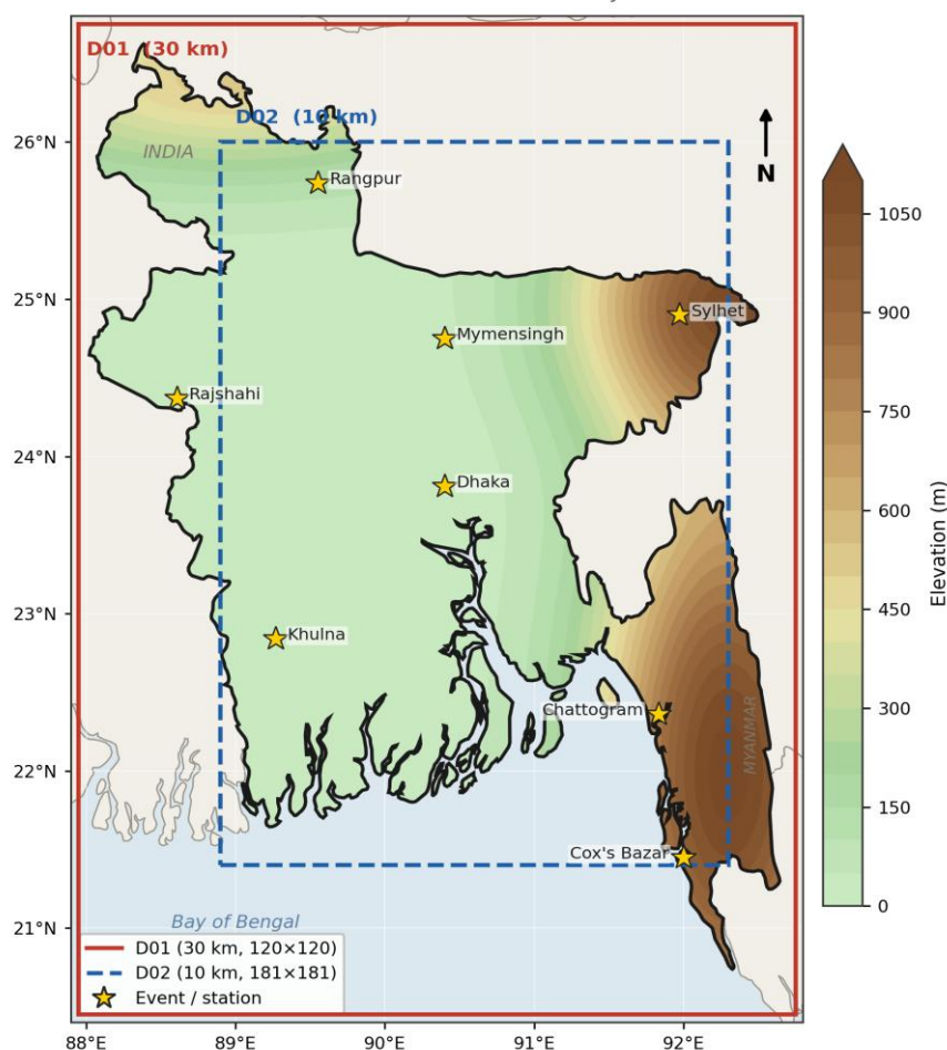
Figure 1. Bangladesh study area showing terrain elevation, the two nested WRF-Chem model domains (D01: 30 km; D02: 10 km), neighboring countries, the Bay of Bengal, and selected heavy-rainfall event / station locations.
