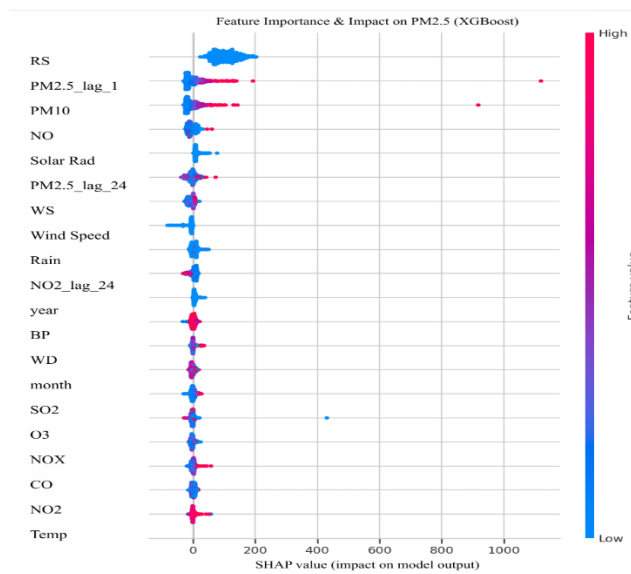
Fig. 3. SHAP-Based Feature Importance Analysis
